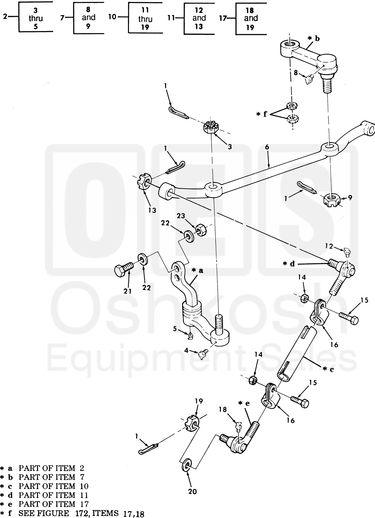
Figure 170. Steering Linkage.
